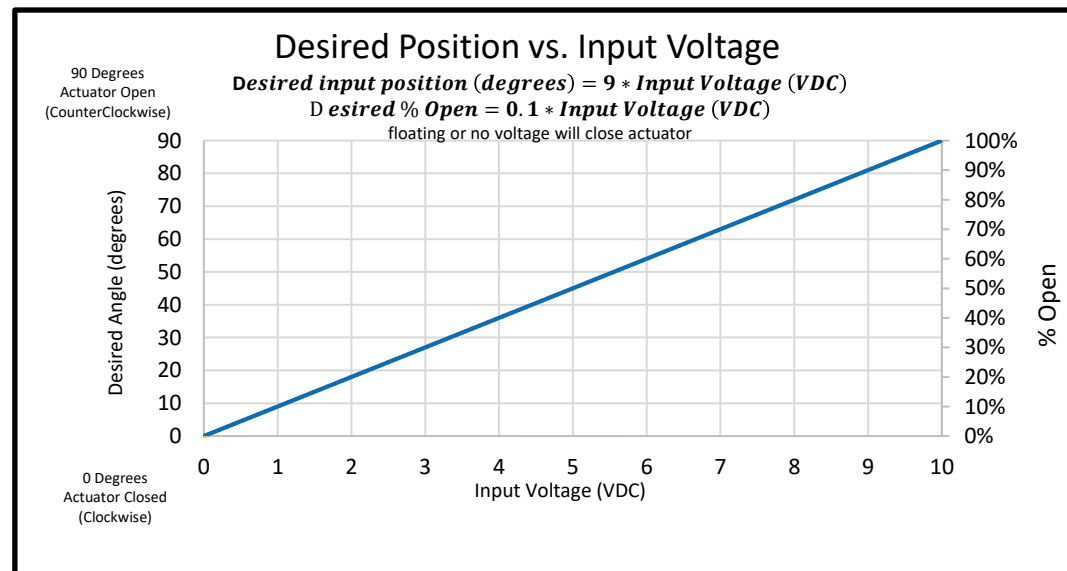
Chart 1: Desired Position vs. Input Voltage
