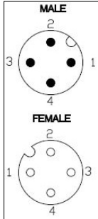
Figure 1: M12 Pinout
